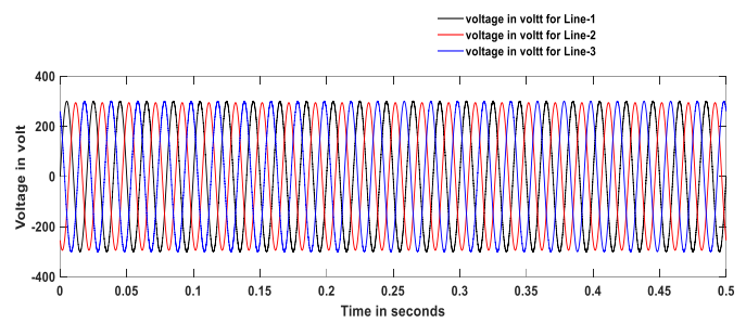
Figure. 6. showing voltage in volt at un equal load
