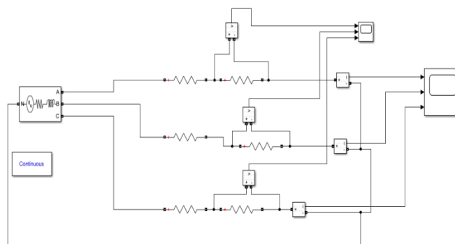
Figure. 3. System modeling under study with resistive load connected.
