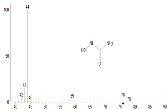
Figure 2. Hydroxyurea detected by GC/MS.
